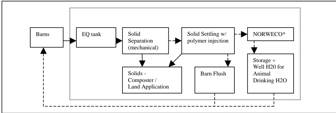
Figure 3. Process flow diagram for Environmental Technologies technology. * NORWECO - This system provides a tertiary treatment to water that will be used as animal drinking water through filtration and aeration.
