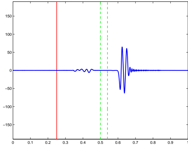
Figure 3(g): E field vs depth – t=4.00025e-9
