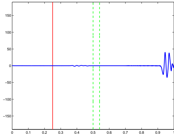
Figure 3(k): E field vs depth – t=6.50025e-9
