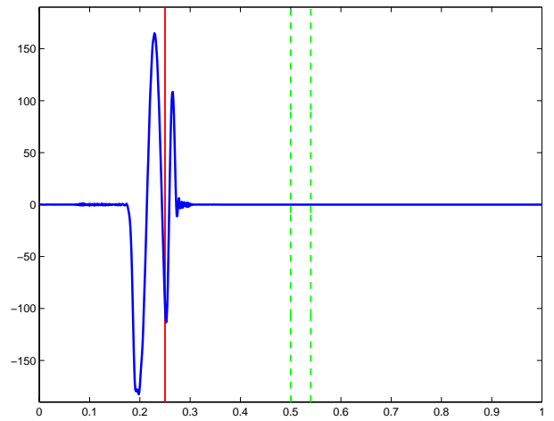
Figure 3(b): E field vs depth - t=1.00025e-9
