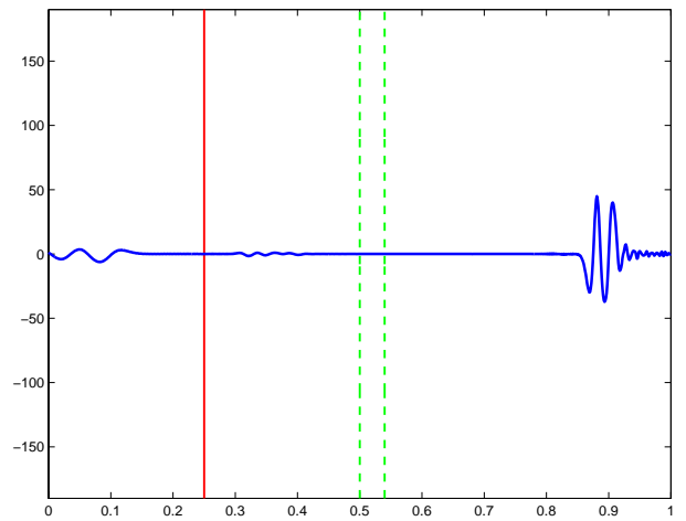
Figure 3(j): E field vs depth – t=6.00025e-9
