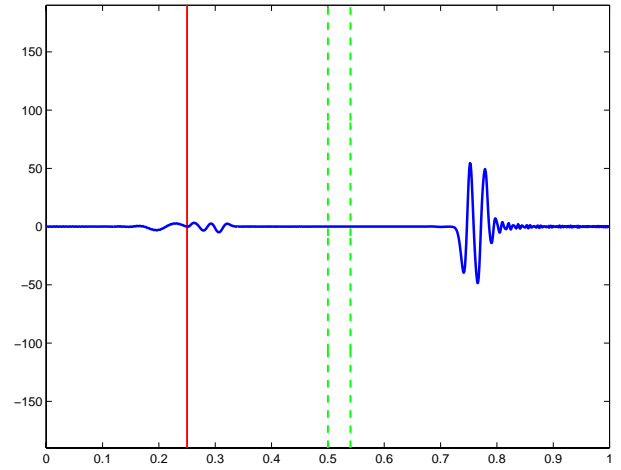
Figure 3(h): E field vs depth – t=5.00025e-9
