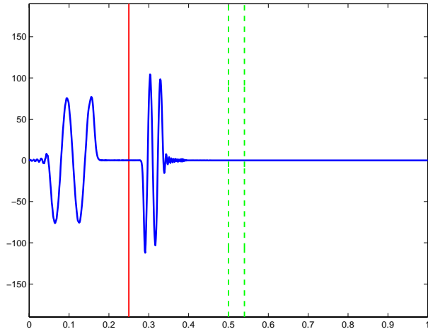
Figure 3(c): E field vs depth – t=1.50025e-9
