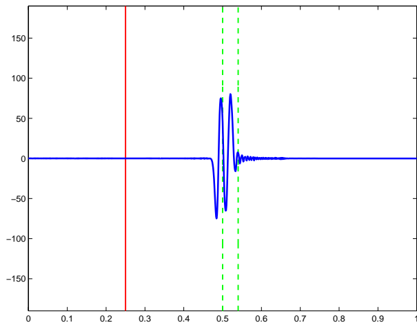
Figure 3(e): E field vs depth – t=3.00025e-9
