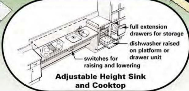
E kitchen counter section with sink and cooktop electrically raises and lowers for comfortable use by all
